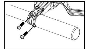
4mm Allen wrench Final tightening torque: 5-7 Nm
